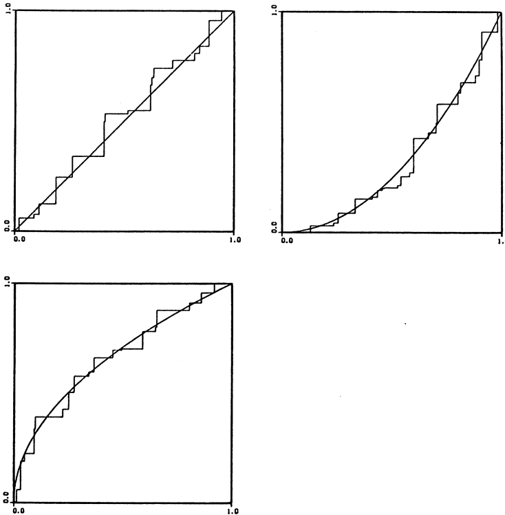
Figure 4.1. The NPMLE computed for samples of size 1000.
